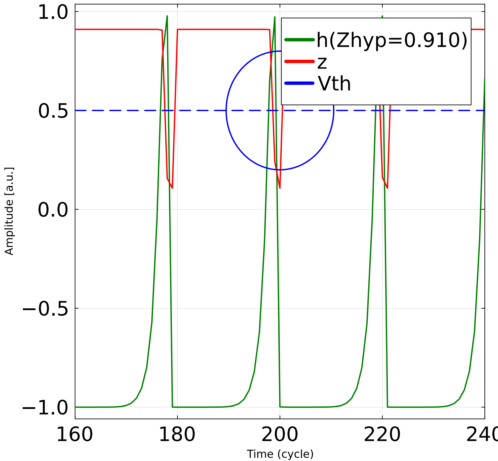
Zoom h(Z_{hyp}=0.910) - V_{th}
